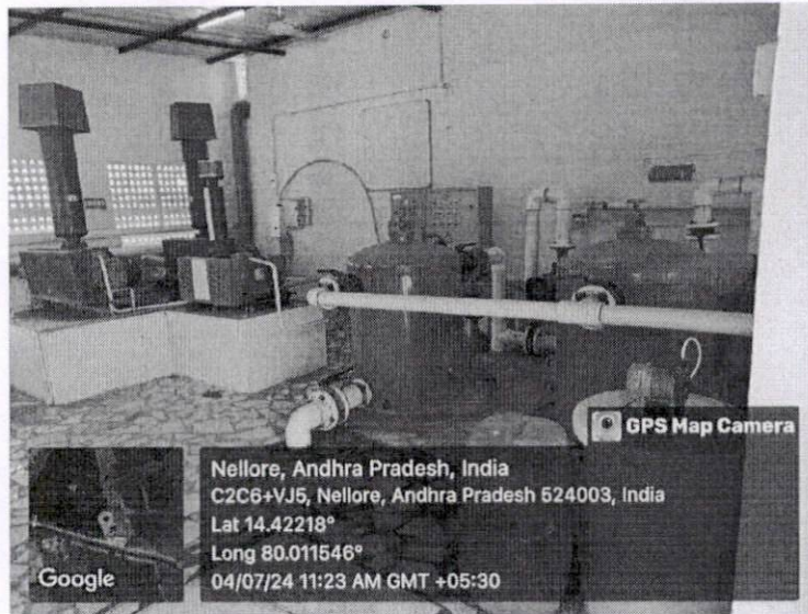
Geotagged photo of inside of sewage treatment plant
