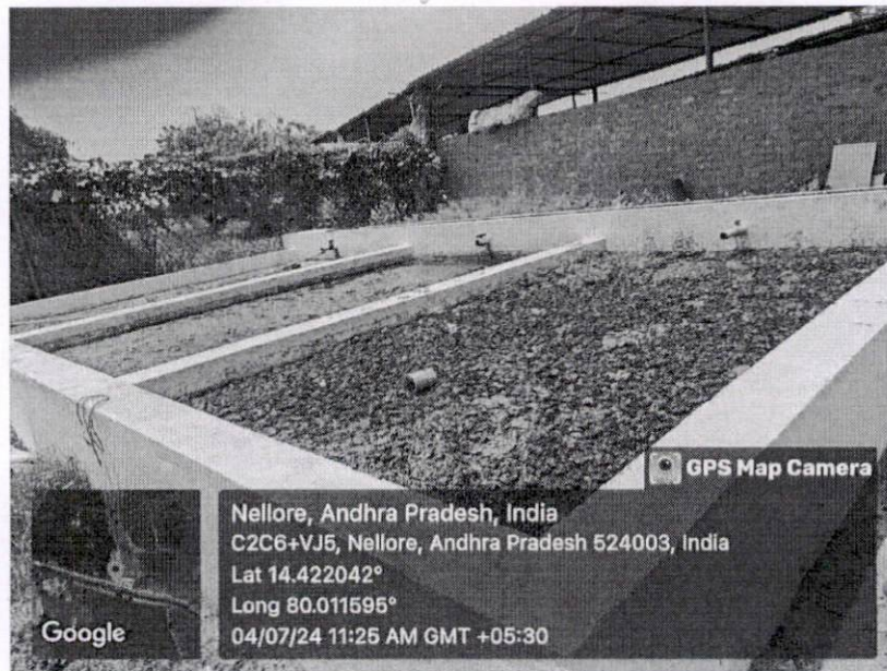
Geotagged photo of Dry beds for dewatering the sludge
